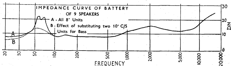
FIG. 9/15.—Impedance curves of multi-speaker system described in text.
