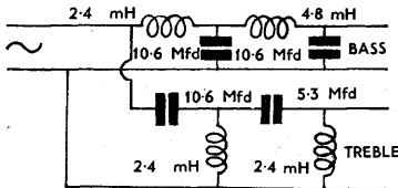
N.W.9. Full Section Parallel Network
