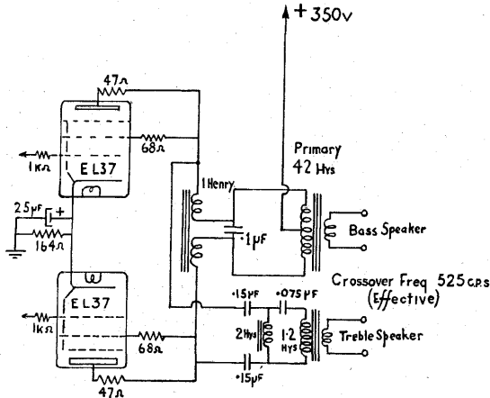
FIG. 45/2.—High Impedance crossover network, as used with Ambassador Corner Speaker described in "Loudspeakers".
