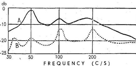
FIG. 86.—Vibrations at 8 in. radius.
