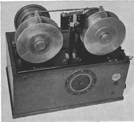
FIG. 48. Poulsen's Telegraphone.
