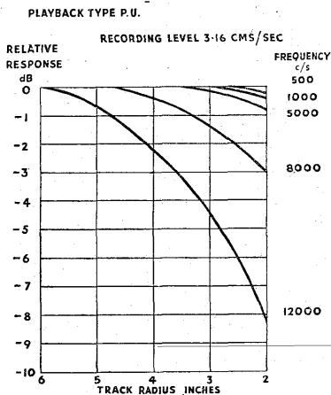
FIG. 58A.—Graph showing relative response at various frequencies at different groove diameters.
