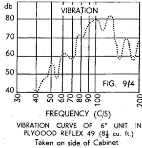
FIG. 9/4. Reflex—Vibration Curves.
