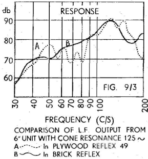
FIG. 9/3. Reflex—Resonance Curves.
