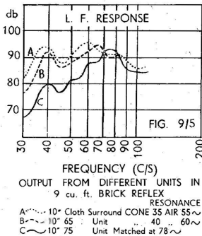
FIG. 9/5 Reflex—L.F. Response.
