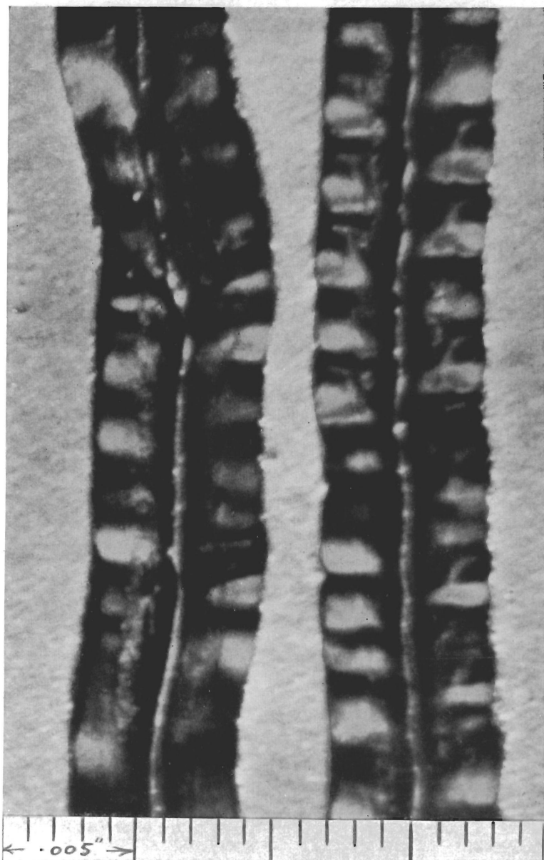
FIG. 73C.—Section of "Danse Macabre" record after 200 playings with crystal pick-up at 7\frac{1}{2} grammes.
