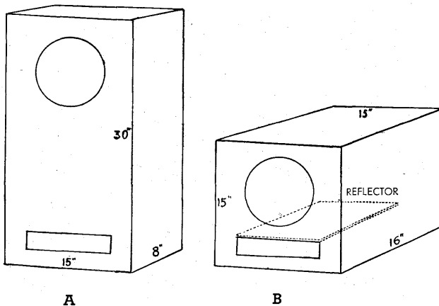
FIG. 2A and 2B.—Reflex cabinets with 8" unit. Same volume—different shape.
