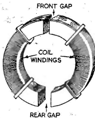
FIG. 48/7.—Magnetic Transducing Head for recording, reproducing or erasing.
