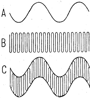
FIG. 48/13.—Application of H.F. bias. A—Audio signal B—H.F. bias C—Combination wave
