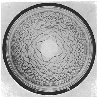
FIG. 93.—Stator with wave formation of required tonal characteristics.
