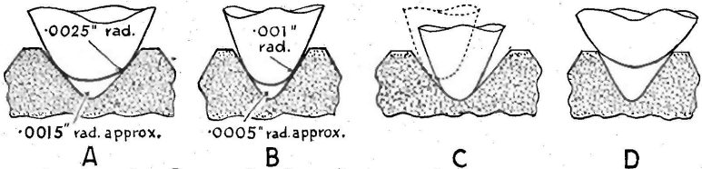
FIG. 63.—A. Correct fit of needle in standard groove. B. Correct fit of needle in microgroove. C. Needle too fine for groove. D. Needle too big for groove.
