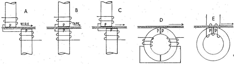
FIG. 48/4.—Various methods of magnetisation.
