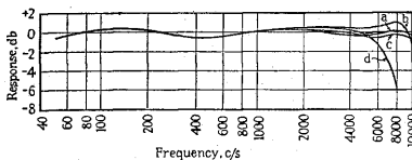
FIG. 62.—Overall frequency characteristics of B.B.C. records.
