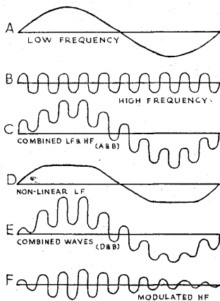
FIG. 43/I.—Typical wave formations showing effect of Intermodulation.
