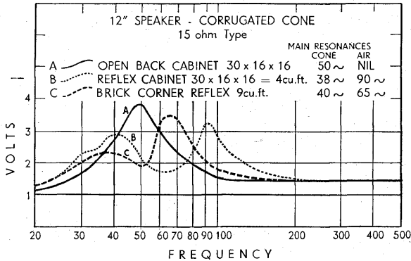
FIG. 1.—Bass Resonance.
