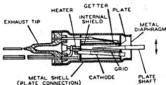
FIG. 87/I.—Electronic Pick-up.
