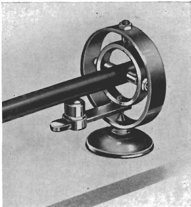
FIG. 89. Tone-arm mounting used for Leak moving coil pick-up.
