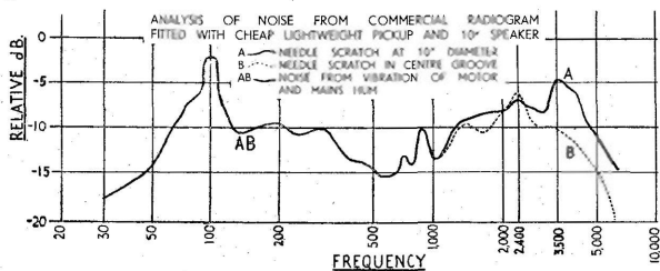
FIG. 81.—Commercial radiogram.
