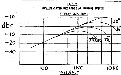
FIG. 48/9.—Uncompensated response of E.M.I. Tape 2 at various speeds, with replay gap 0.00055".
