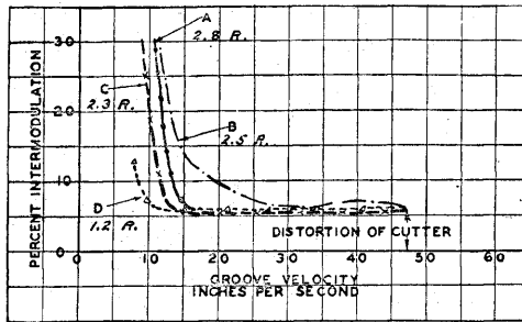
FIG. 43/2. Intermodulation distortion with pickups of different tip radii, in narrow groove.
