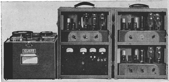
FIG. 17.—Magnetic recorder with 3 amplifiers for stereophonic reproduction of sound.
