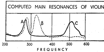
FIG. 45.—Computed main resonances of violin.
