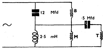
N.W.10. Three Speaker circuit. Crossover at 1000 & 5000 cycles
