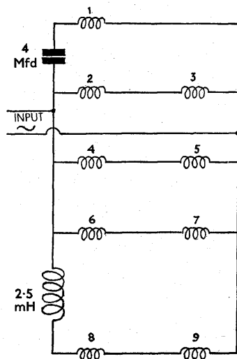
FIG. 9/14.—Circuit diagram of multi-speaker system described in text.
