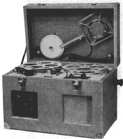
FIG. 50/2.—The Sound Magnet, Tape Recorder.
