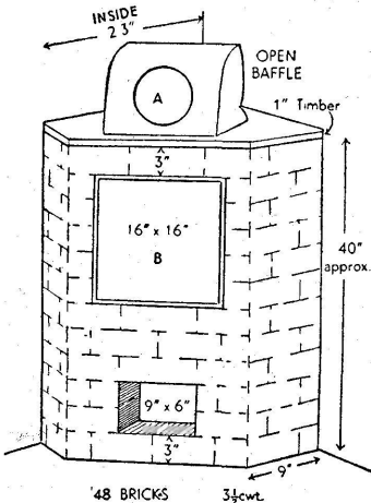
FIG. 30. — Non-resonant corner Reflex for bass. Capacity 9 cu. ft. Small open baffle reflecting into corner for treble.
