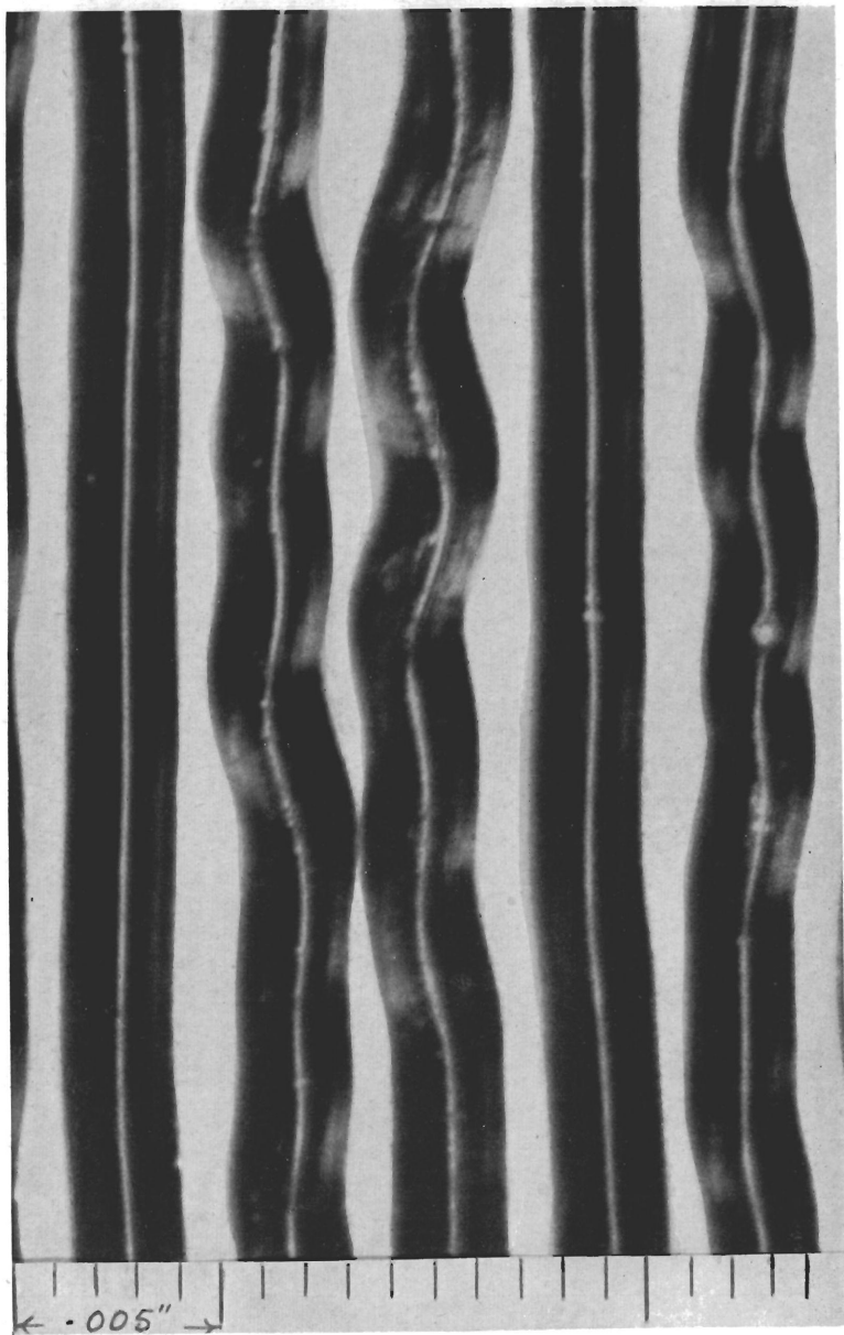
FIG. 91D.—Same record as 91C after 300 playings with crystal pick-up and sapphire, tracking at 5 grammes.
