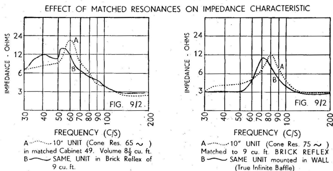
FIG. 9/2. Impedance—matched Resonance.
