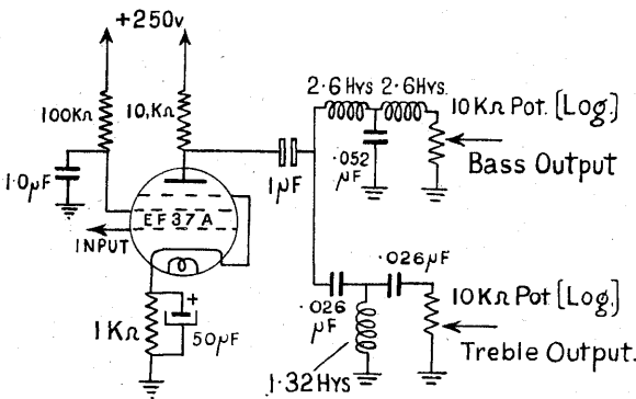
FIG. 45/1.—T-section Filters for independent Bass and Treble Amplifiers.
