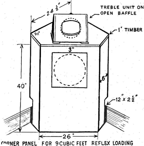
FIG. 31.—Diagram of panel to replace brick of Fig. 30.
