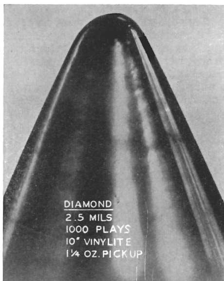
FIG. 62/5.—Photograph of Diamond after 1,000 playings at 78 r.p.m.
