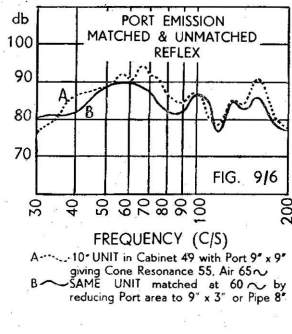
FIG. 9/6. Reflex—L.F. Response.
