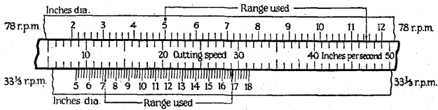
FIG. 60 Cutting speed at various recording diameters.
