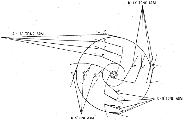
FIG. 79.—Tracking Error.
