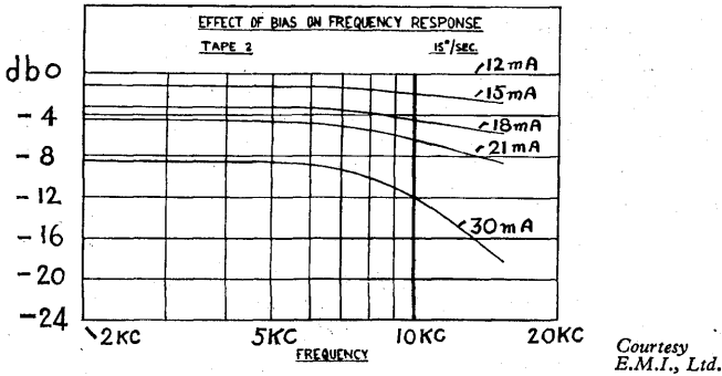
FIG. 48/15.—Effect of bias on frequency response.
