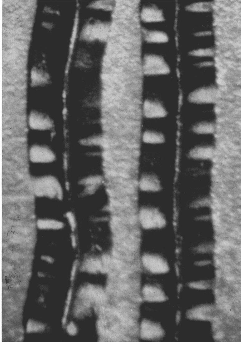
MODERN SHELLAC DISC AFTER TWENTY PLAYINGS WITH SAPPHIRE IN APPROVED LIGHT-WEIGHT PICKUP
