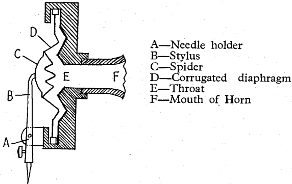
FIG. 53.—Mechanical Soundbox.
