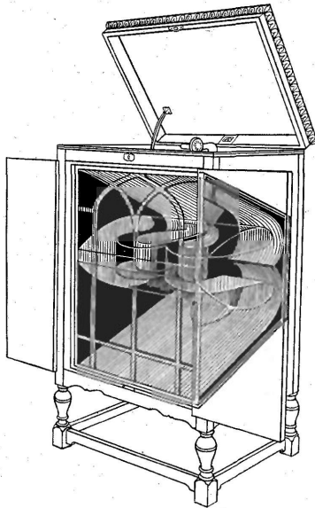
FIG. 55.—Re-entrant Exponential Gramophone.
