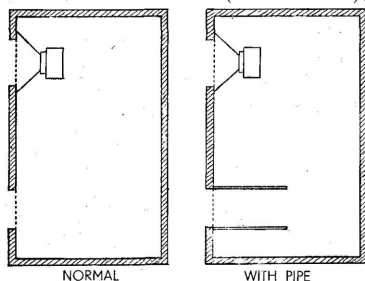
REFLEX CABINETS (SIDE VIEW)
